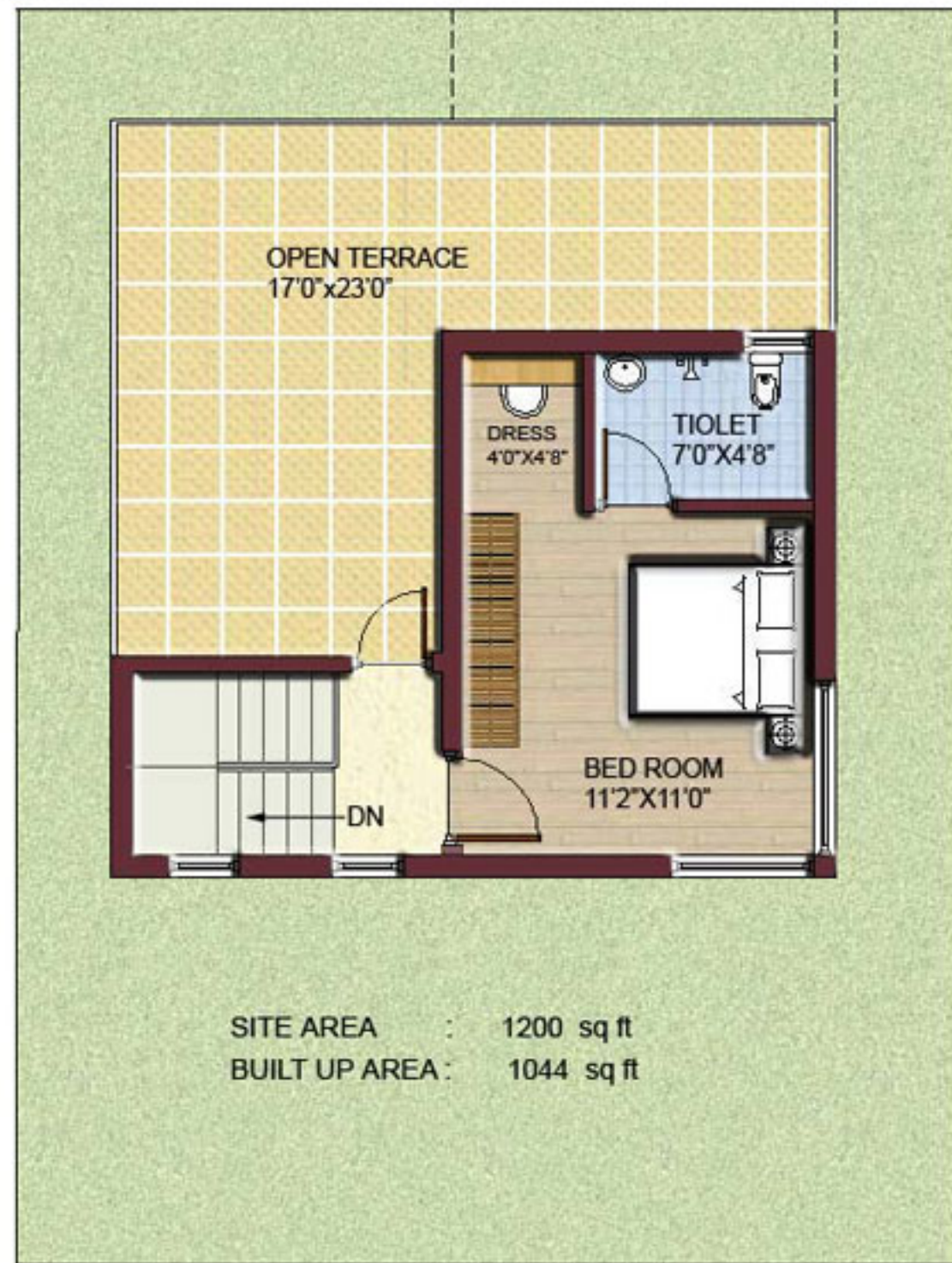
FIRST.FLOOR
