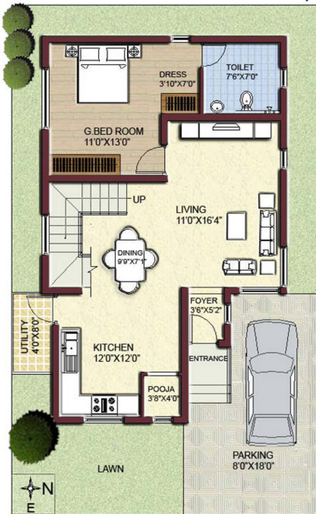
GROUND.FLOOR
