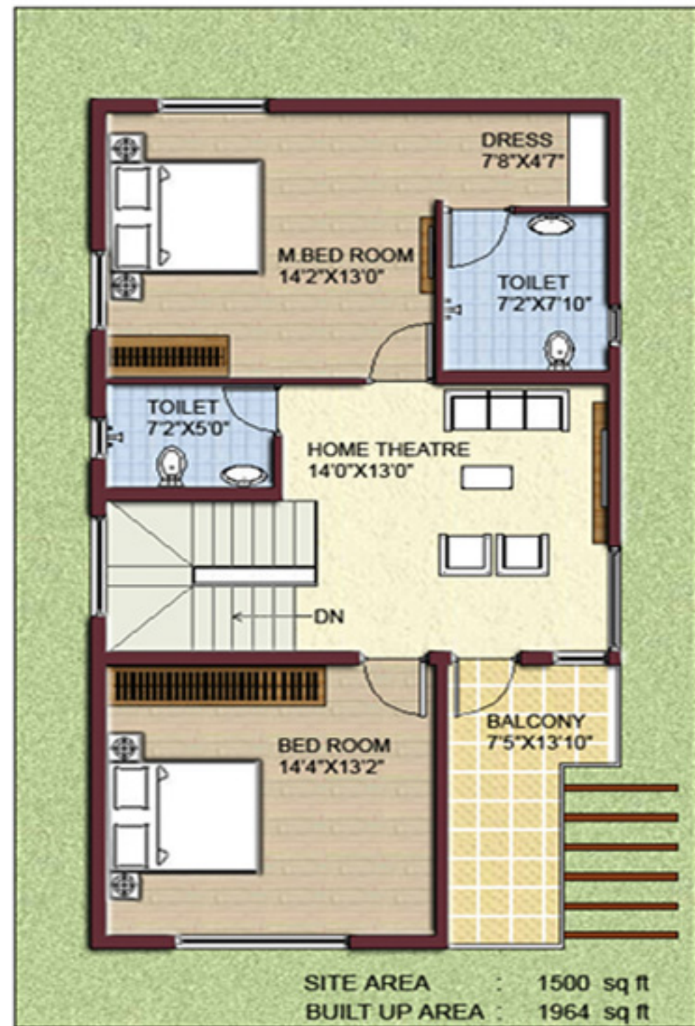
FIRST FLOOR
