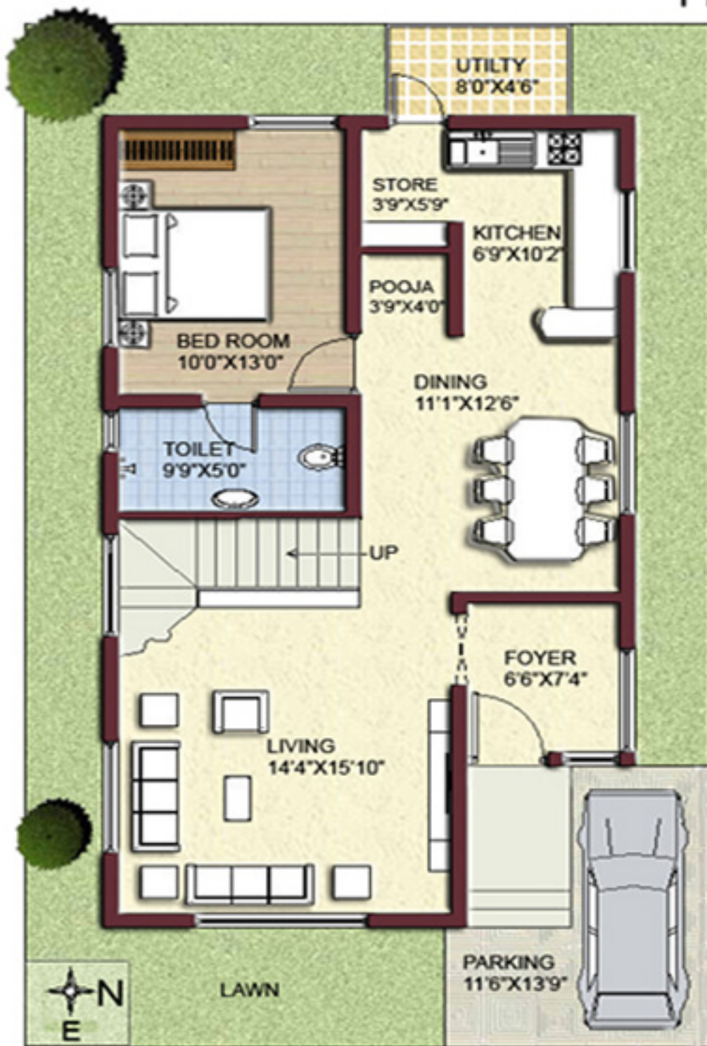
GROUND FLOOR
